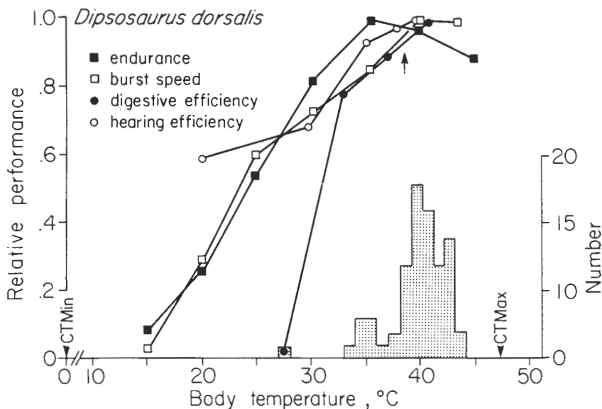
Figure 3 Sensitivity of several physiological functions to body temperature in a lizard, the desert iguana Dipsosaurus dorsalis . The body temperatures of lizards in nature (histogram) or in a laboratory thermal gradient (up arrow) enable the lizards to perform at or near maximal physiological capacities. Critical thermal limits (loss of righting response) are also shown (down arrow). Original sources of data in Huey (1982). (Modified, with permission, from Huey 1982.)
