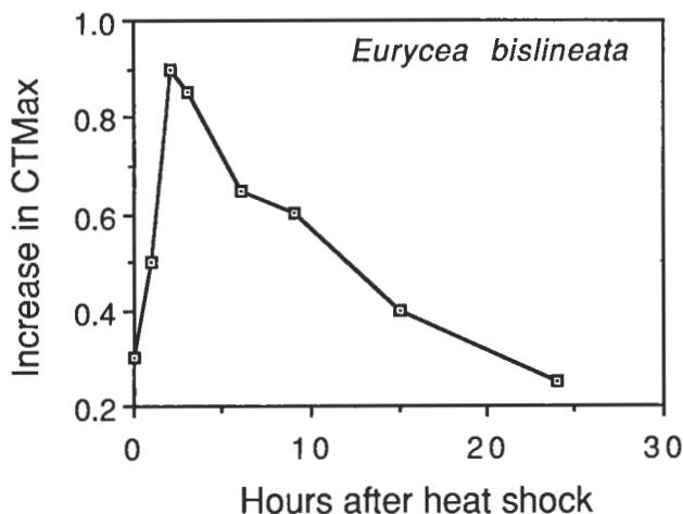
Figure 4 Heat hardening (i.e., increase in critical thermal maximum, CTM, measured as onset of spasms) in the salamander Eurycea bislineata following a 1-hr exposure to a temperature 2°C below an individual's (previously established) CTM. (Modified, with permission, from Easton et al. 1987.)
