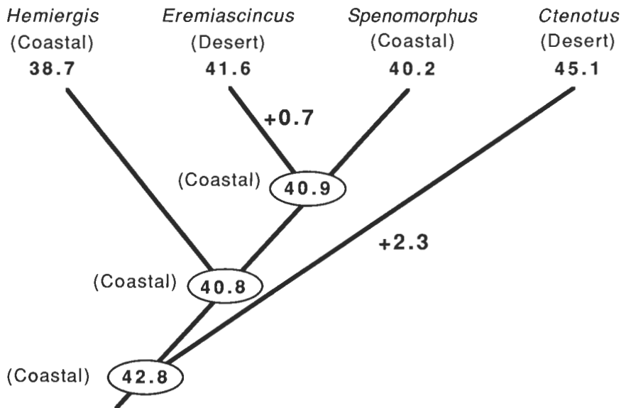
Figure 7 A partial phylogeny of some Australian lizards (Scincidae), showing critical thermal maxima (loss of righting response) and current habitat associations (desert vs. coastal) for the different genera and for their presumed ancestors. (Intragenetic variation in critical thermal maxima is minor in these lizards.) The values of hypothetical ancestors are estimated using an algorithm that minimizes the evolutionary change in the tree (see text). Note that the invasion of the Australian desert by two genera ( Eremiascincus , Ctenotus ) is associated with an apparent increased heat tolerance (critical thermal maximum). From data in Huey and Bennett (1987).
