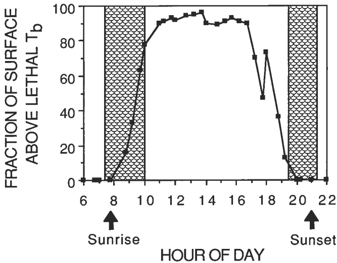
Figure 1 On a clear summer day in Big Bend National Park, Texas, equilibrium body temperatures for the canyon lizard ( Sceloporus merriami ) would exceed the lizard's lethal temperature on most of the ground surface. Lizards restrict their activity on the ground surface to early and late in the day ("scaly" regions). (Original data courtesy of B.W. Grant and A.E. Dunham.)
