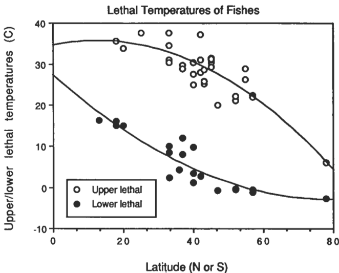
Figure 6 Upper and lower lethal temperatures for fishes (post-embryonic states only) from different latitudes. Curves fitted by polynomial regression. (Redrawn, with permission, from Brett 1970.)
