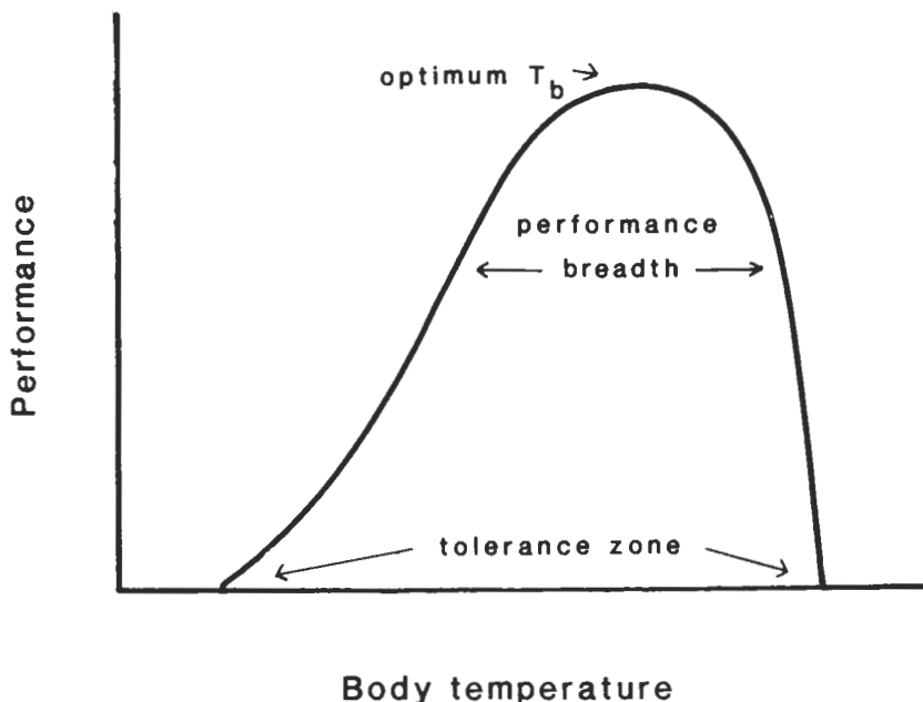
Figure 2 Effect of body temperature on the physiological performance capacity of a hypothetical ectotherm. (Modified, with permission, from Huey and Stevenson 1979.)
