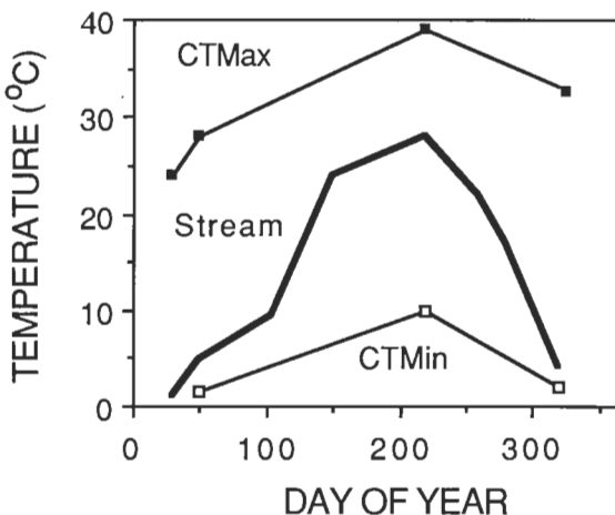
Figure 5 Critical thermal limits of the crayfish Orconectes rusticus and water temperatures at different seasons. Note the parallel shifts in critical limits and in water temperatures. (Redrawn, with permission, from Layne et al. 1987.)
