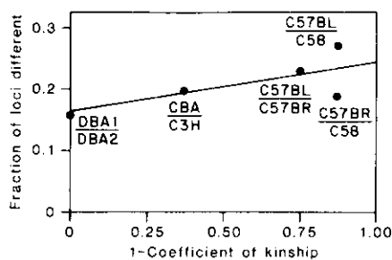
Fig. 3. Plot of d_{ij} as a function of c_{ij} from the equation d_{ij} = c_{ij}h(1 - 2my_{ij}) + 2my_{ij} with y_{ij} = 58 years. The linear regression gives d_{ij} = 0.079 (\pm 0.043)(c_{ij}) + 0.165 (\pm 0.029) . Distances are from Table 1 adjusted to 58 years (age of the C57 and C58 separation).
